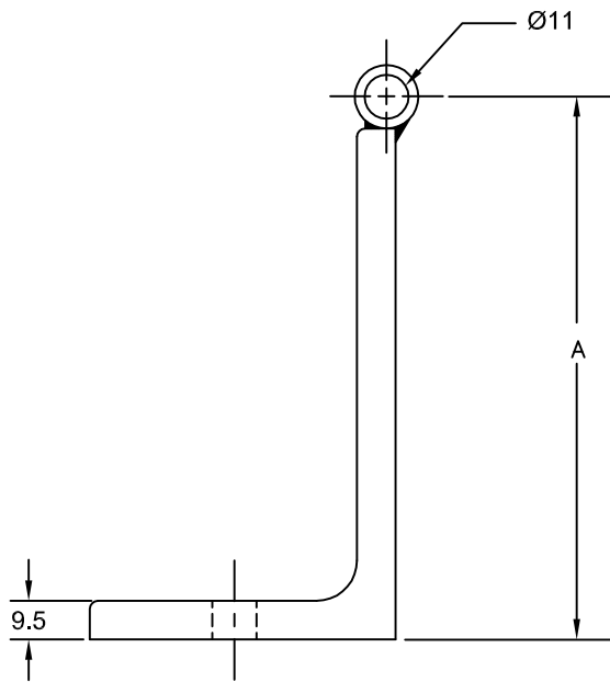
HORIZONTAL STORAGE OR HINGE BRACKET
