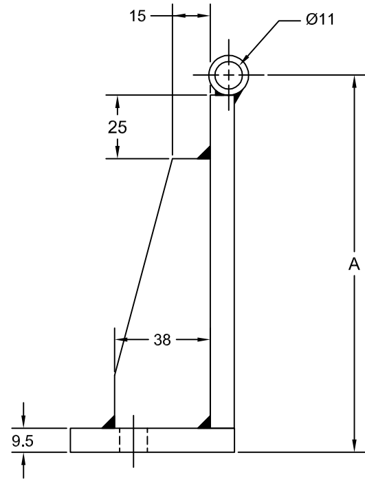
HORIZONTAL EXTENDED STORAGE OR HINGE BRACKET
