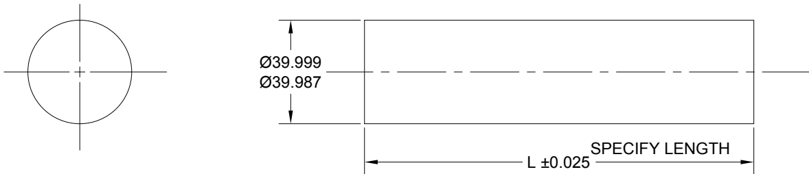
LIFTER SHAFT
