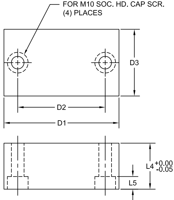
UPPER SHOE 90.30.135-XXXB
