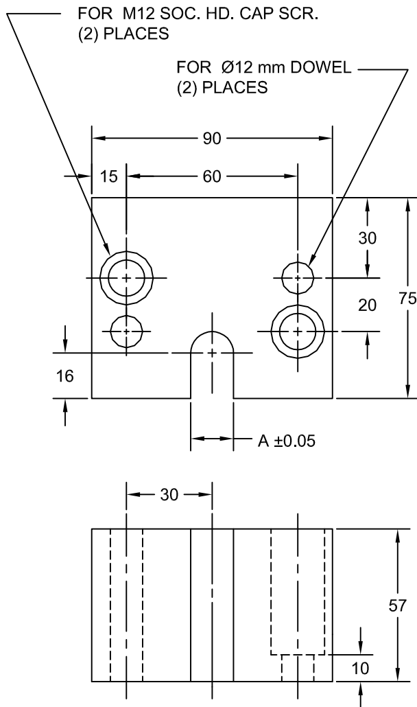
PILOT PIN TRIM BLAD
