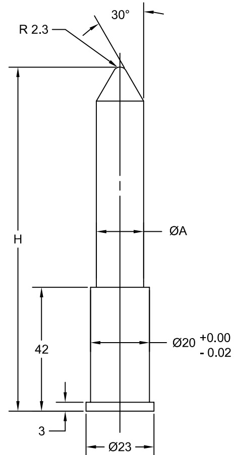
TRIM TAB PILOT PIN
