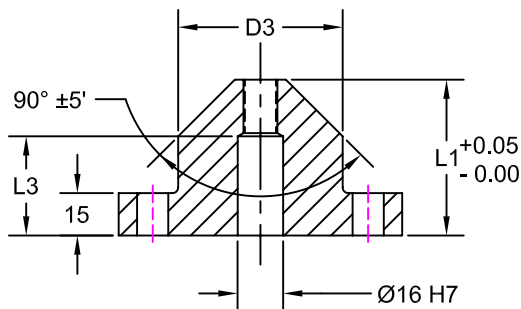
FORM "A" SECTION A-A
