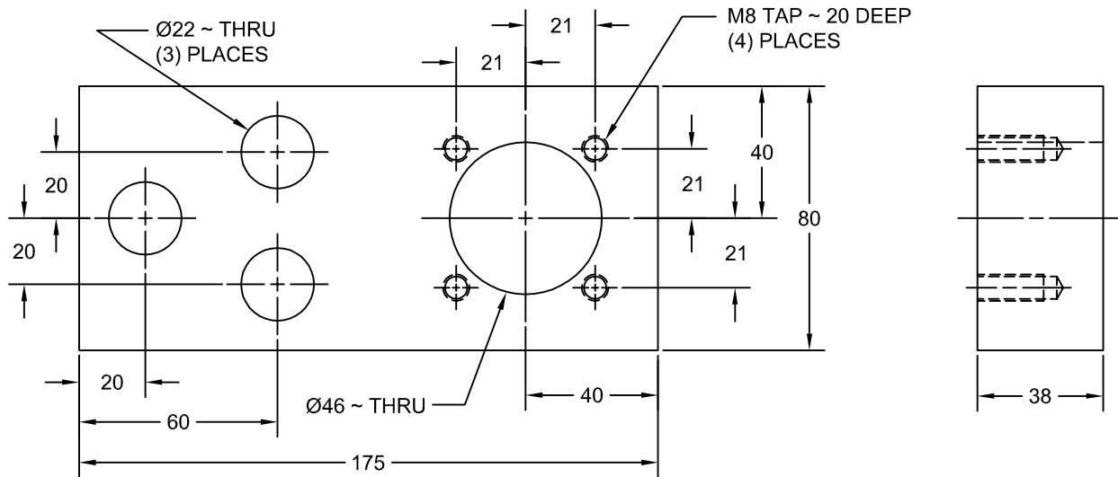
RETAINER PLATE FOR SINGLE PAD DAMPER
