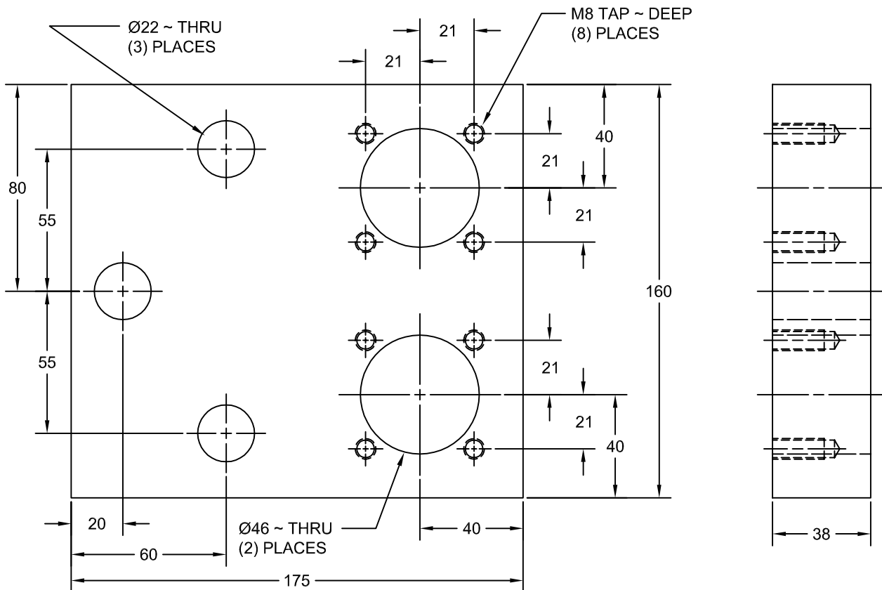
RETAINER PLATE FOR DOUBLE PAD DAMPER
