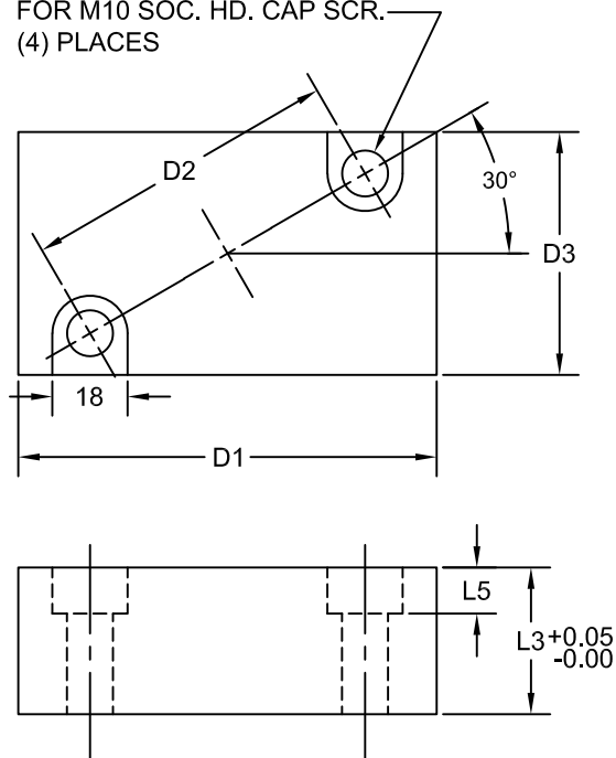
LOWER SHOE 90.30.135-XXXA
