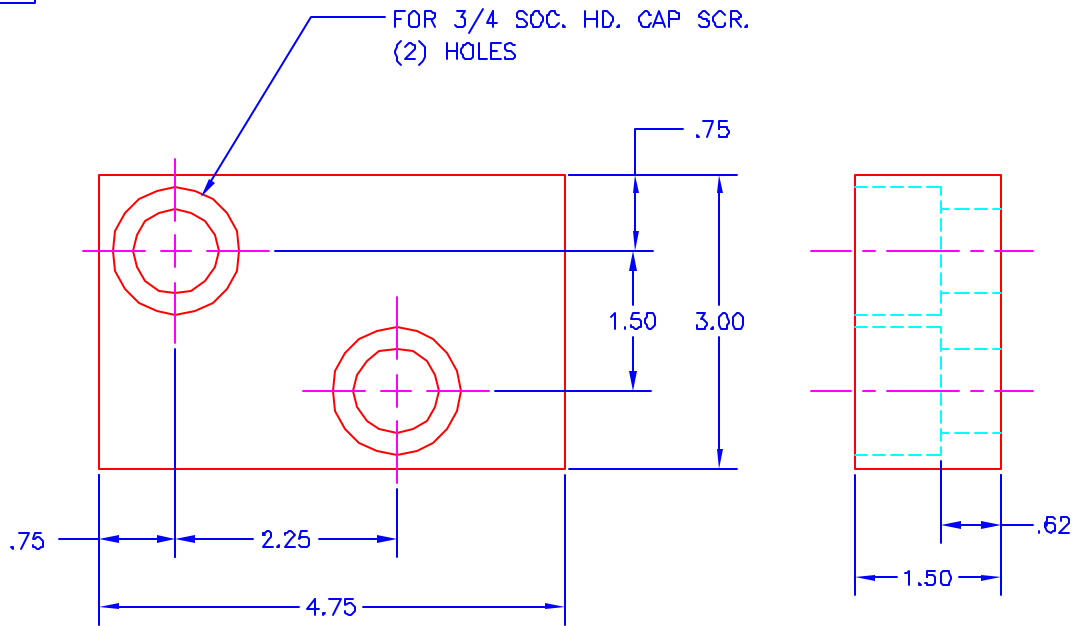
COVER PLATE
