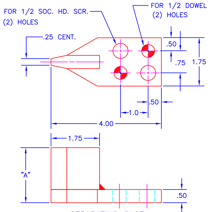
SEPARATING GAGE
