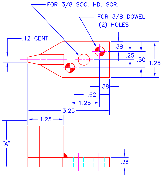
SEPARATING GAGE
